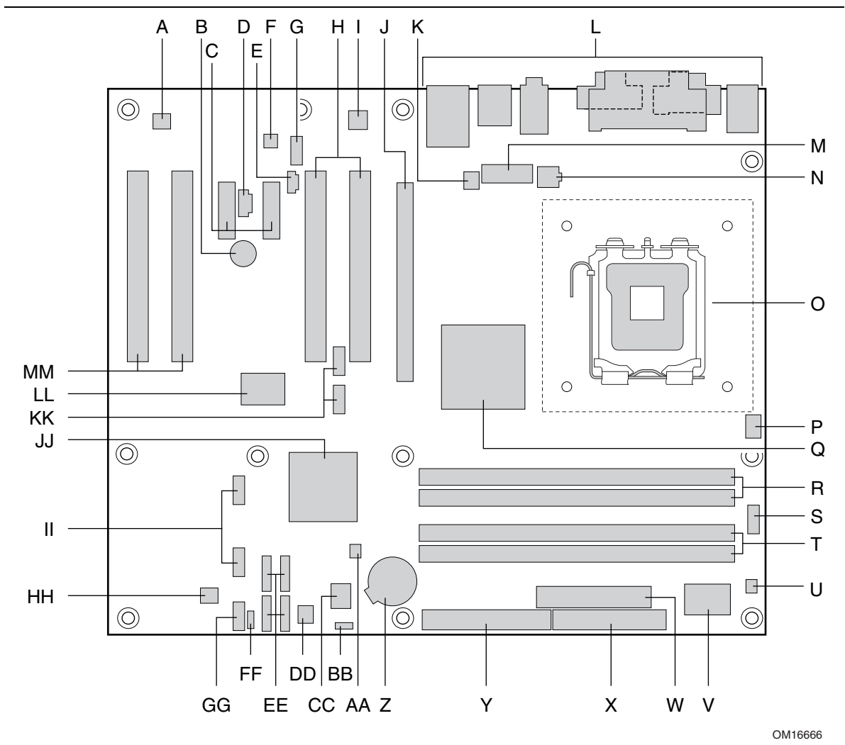
Figure 1. D915GAV Board Components
