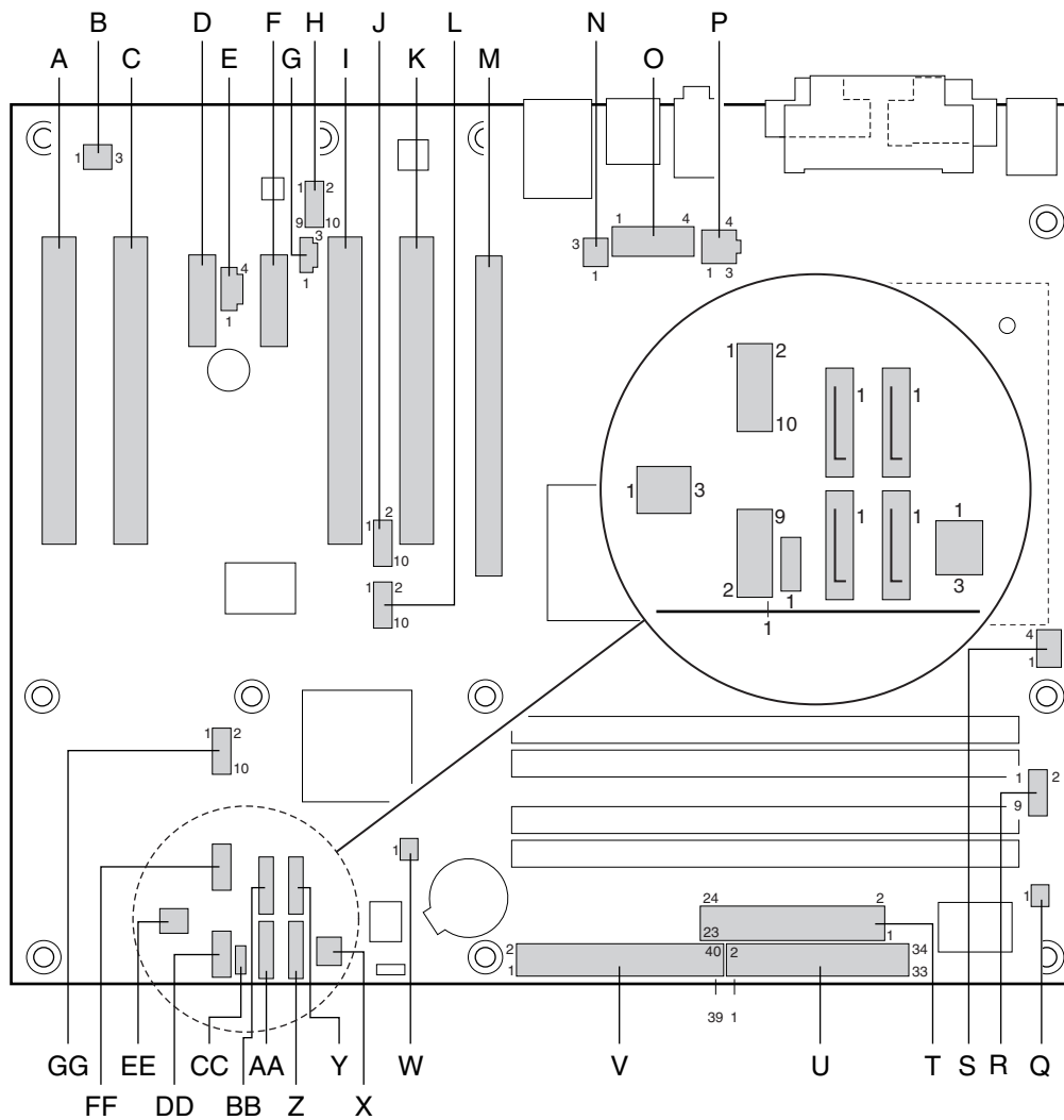
Figure 18. D915GAV Board Component-side Connectors
