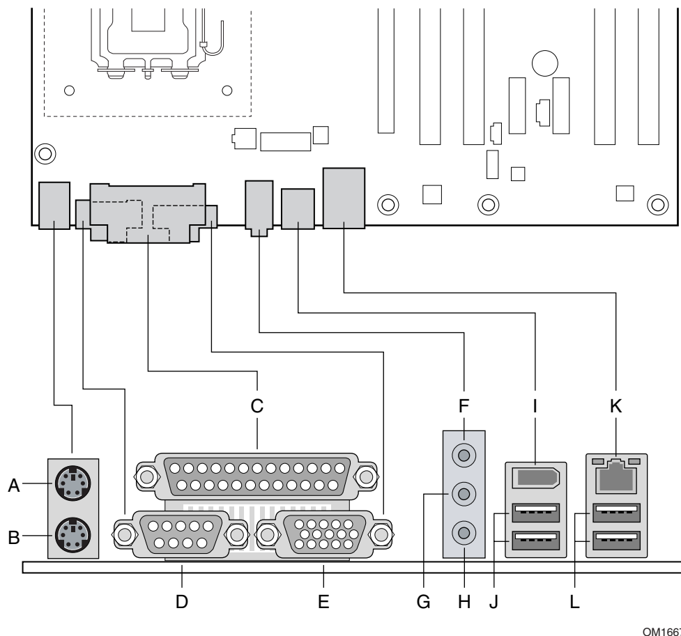
Figure 17. Back Panel Connectors
