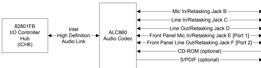
Figure 11. High Definition Audio Subsystem Block Diagram
