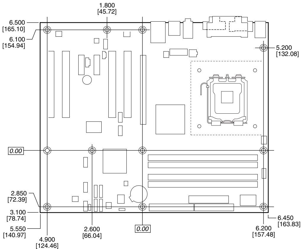
Figure 24. D915GAV Board Dimensions
