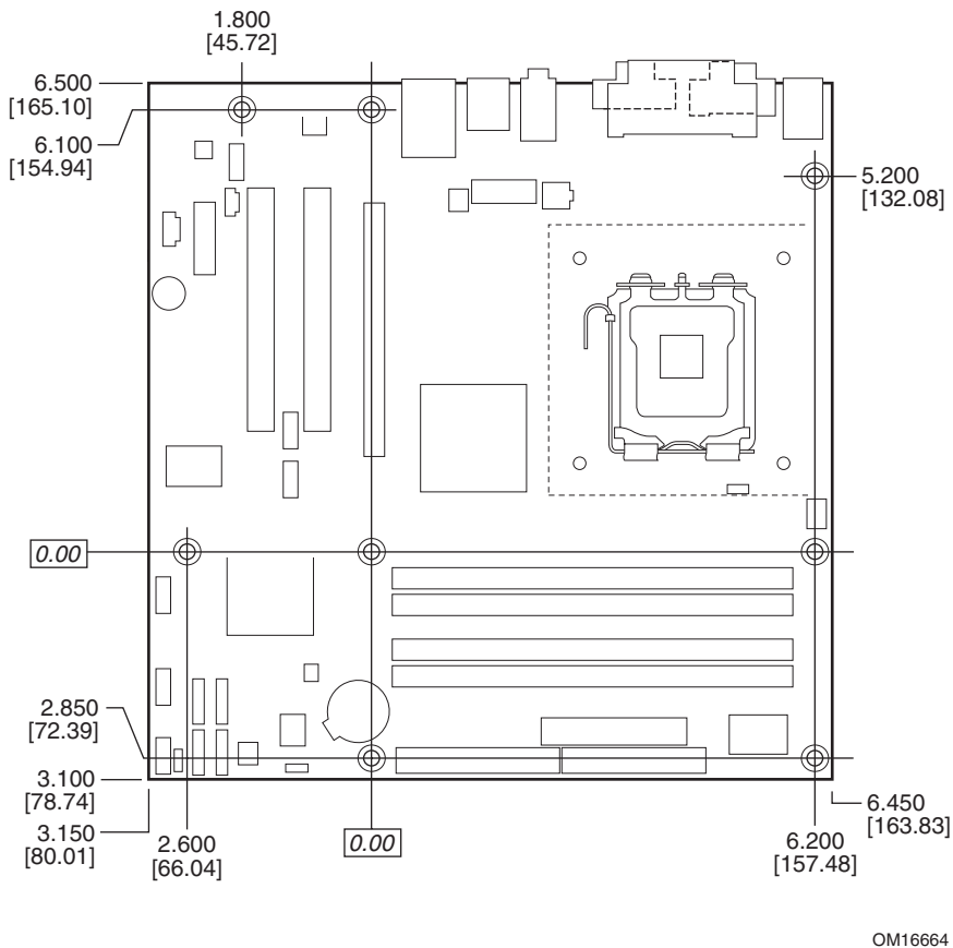
Figure 25. D915GAG Board Dimensions
